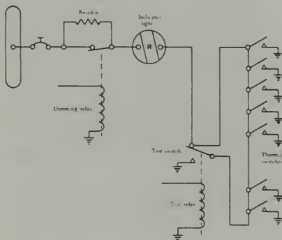
FIGURE 9-1. Thermal switch fire circuit.
